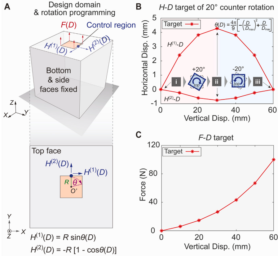
Fig. 2. Problem setup for programming 3D rotation-then-counter-rotation behavior into structures. (A) Design domain, boundary conditions, and control regions; (B) target H - D relation of 20° rotation-then-counter-rotation (a sequential clockwise then counter-clockwise rotation in the horizontal plane); (C) target stiffening F - D relation.
