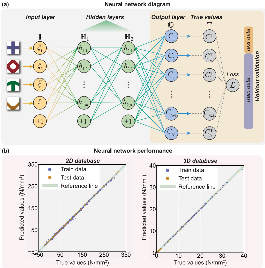
Fig. 4. Neural network diagram for predicting the elasticity tensor based on the input frequency hints. Panel (a) shows a fully connected neural network containing one input layer ( I ), two hidden layers ( H_1 and H_2 ), and one output layer ( O ). The predicted independent components of the elasticity tensor ( C_1 to C_N ) from the output layer are compared with their corresponding ground truth values ( C_1^T to C_N^T ), and the disparity is quantified using the mean squared error (MSE), denoted as \mathcal{L} . Additionally, a holdout validation strategy is employed to ensure the neural network's accuracy and generalizability by partitioning the data into training and testing sets. Panel (b) highlights the outstanding performance of the neural network by presenting a comparison between the true values and the predicted values across both the training and testing datasets within the framework of 2D and 3D databases.
